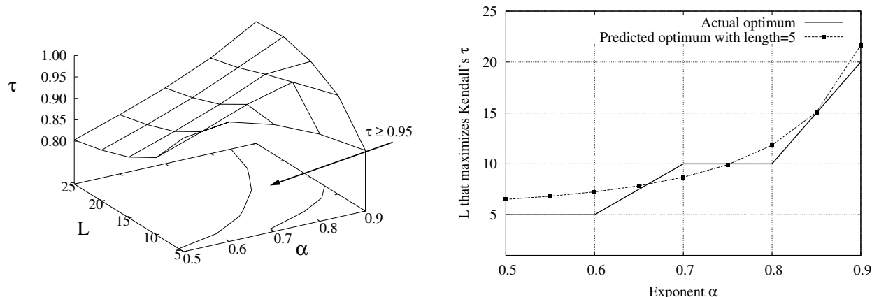
Figure 13: Comparison (using Kendall's \tau ) between PageRank and LinearRank in the U.K. web graph, with various damping parameters. Again, the predicted optimum with \ell = 5 is very close to the actual optimum.
